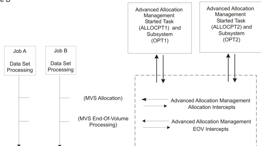
Figure 2. Advanced Allocation Management (multiple instances)
