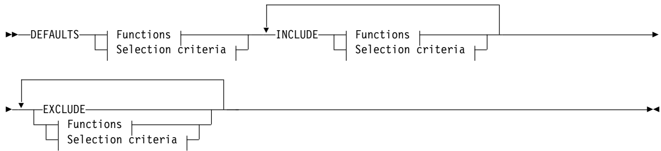
Figure 8. Rule definition syntax
