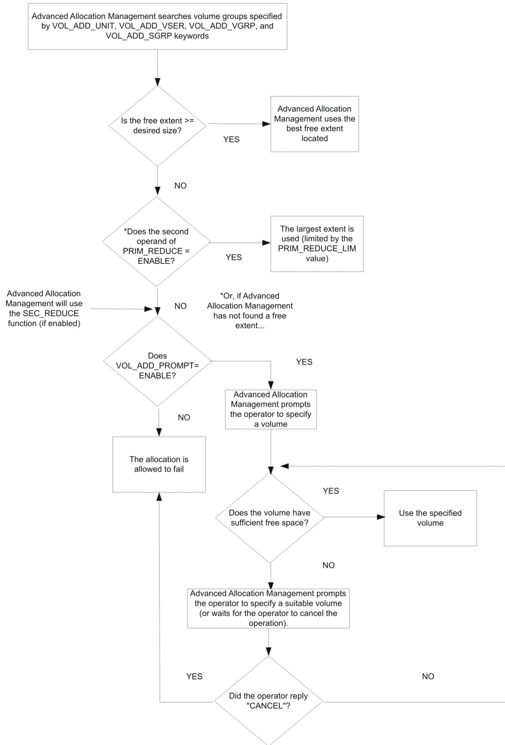
Figure 11. VOL_ADD keyword and associated processing logic
