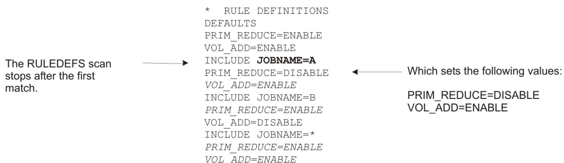
Figure 6. Advanced Allocation Management rule definition processing
